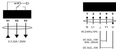
Auxiliary switches
